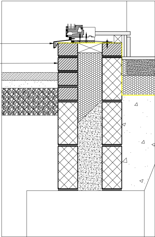
Detailed Section - 1:10
