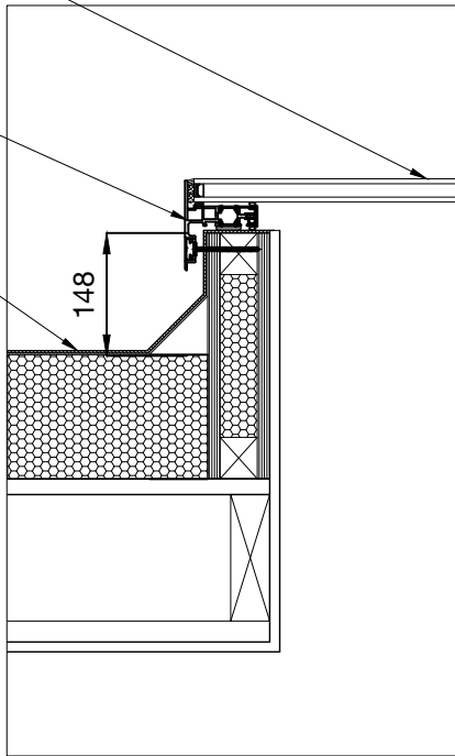
Detailed Section through rooflight. 1:10
