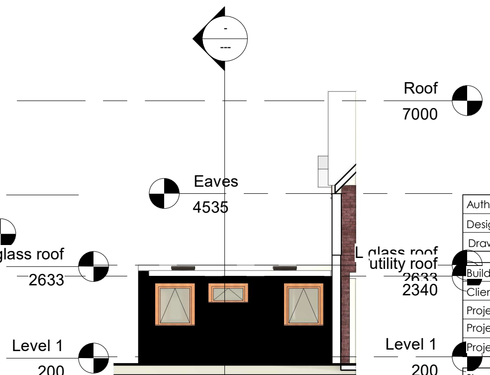
2 Proposed Side Elevation 7 1 : 100
