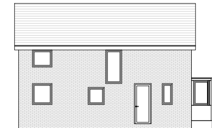
Existing Side Elevation 1:100
