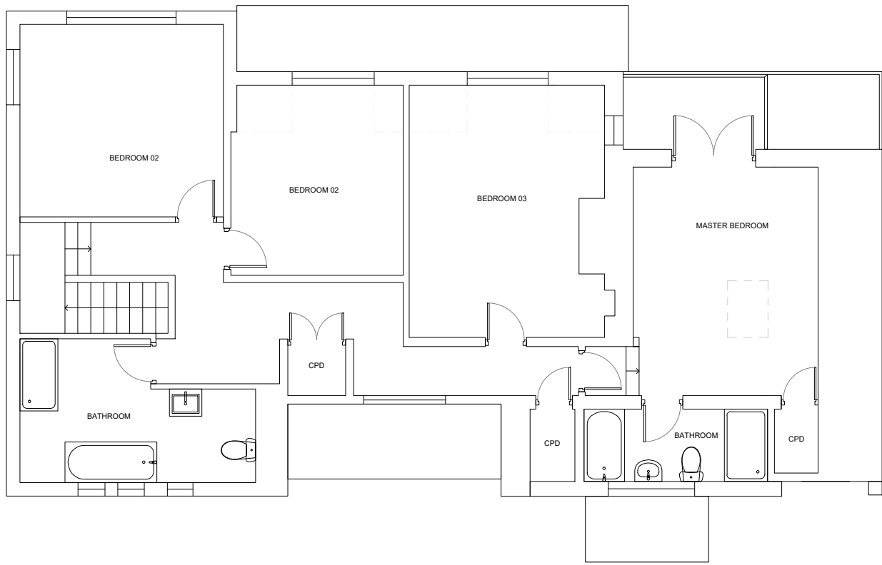
Proposed First Floor Plan 1:100
