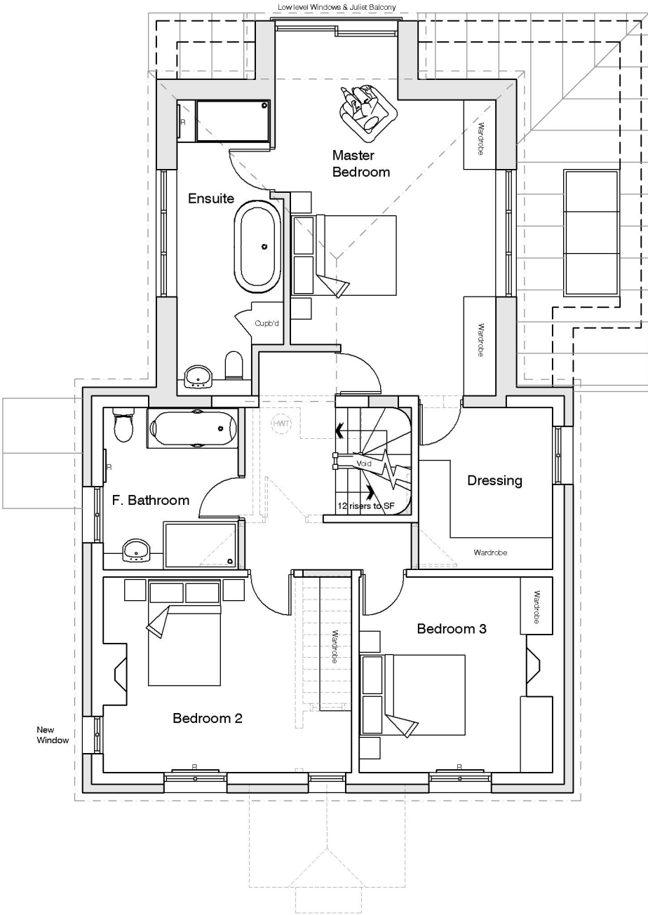
FIRST FLOOR
