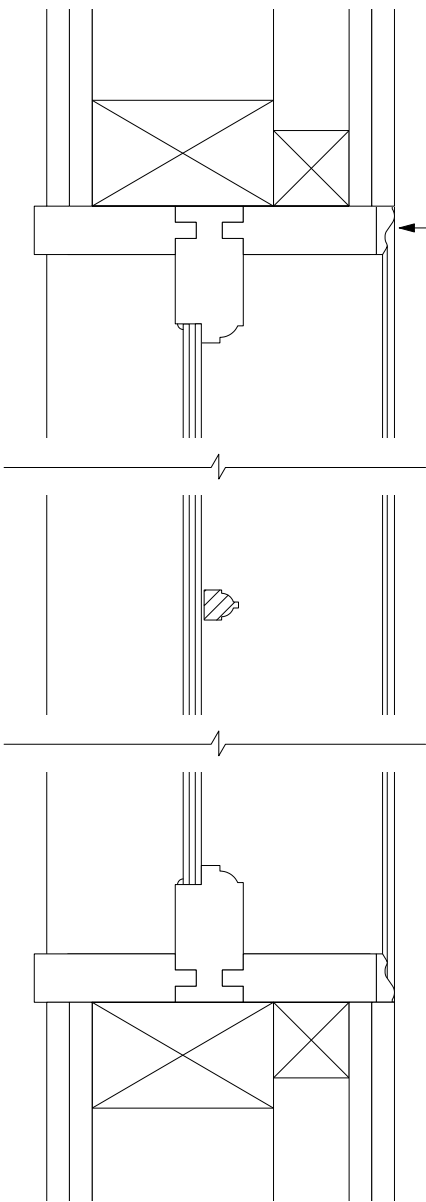
Window Section Detail 1:5 @A3 / 1:2.5 @A1
