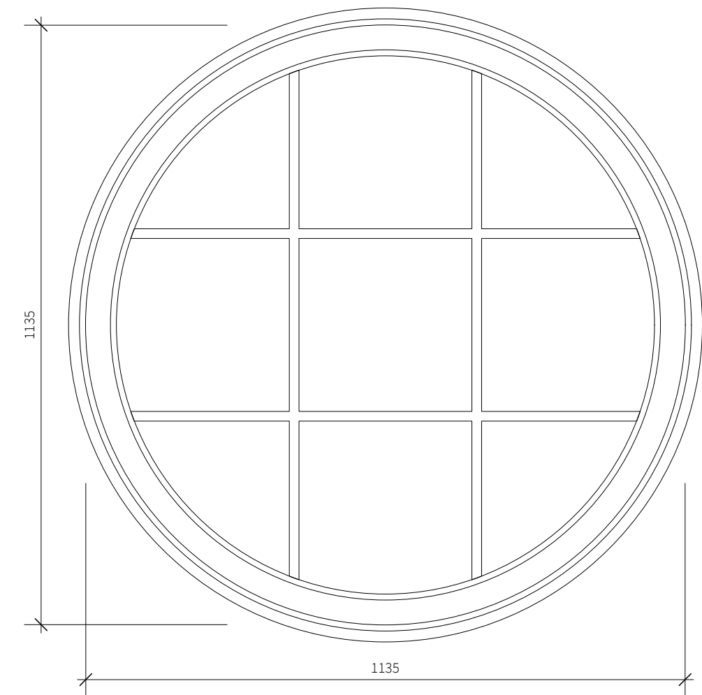
Window Elevation 1:10 @A3 / 1:5 @A1
