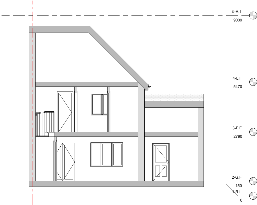
SECTION 2
