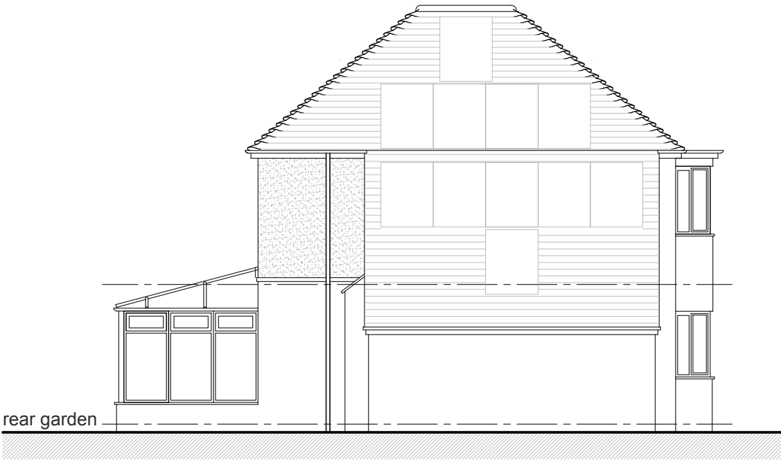
Flank Elevation (east)
