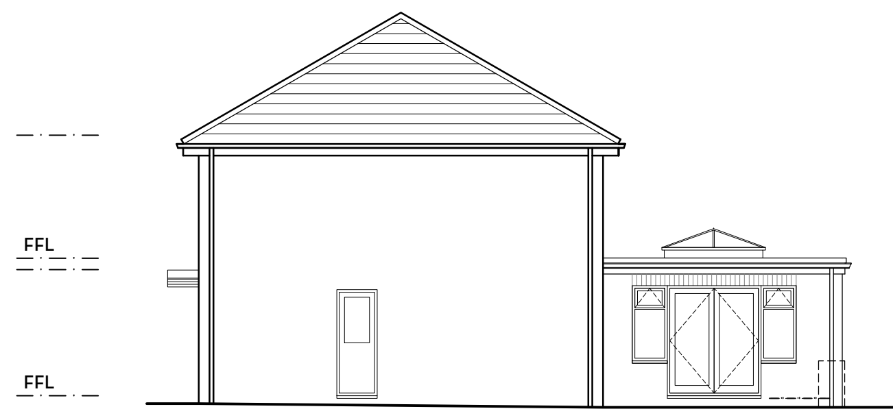
WEST ELEVATION
