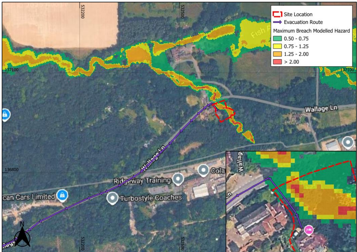
Figure 5: Evacuation Route Overlain Modelled Flood Hazard (Base map from Google Hybrid and data from Aegaea Modelled Breach Outputs)
