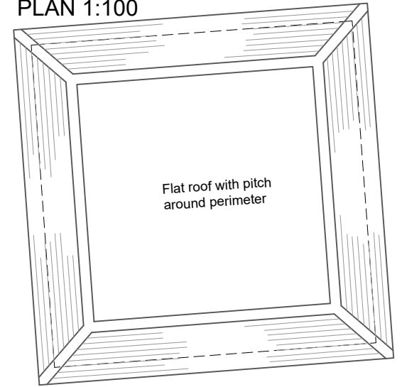
EXISTING GARAGE ROOF PLAN 1:100
