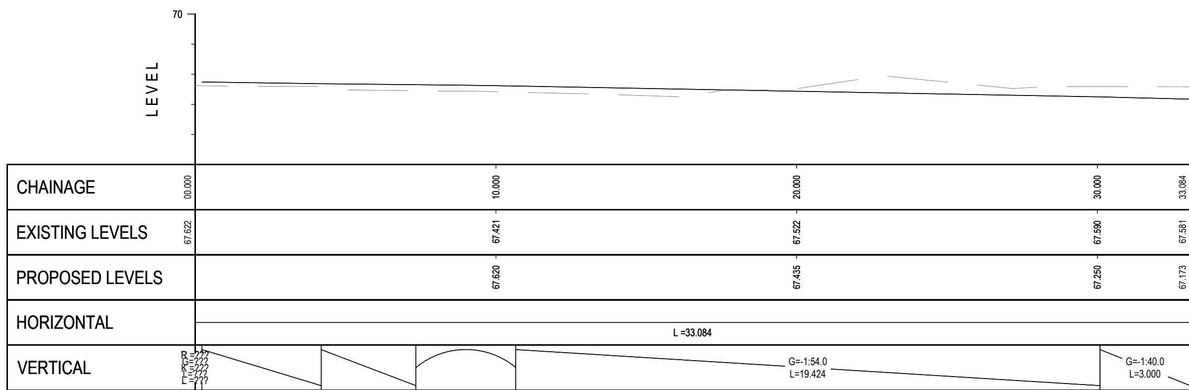
NORTHERN PLOT ACCESS - LONGSECTION SCALE: H 1:500, V 1:500. DATUM: 65.000
