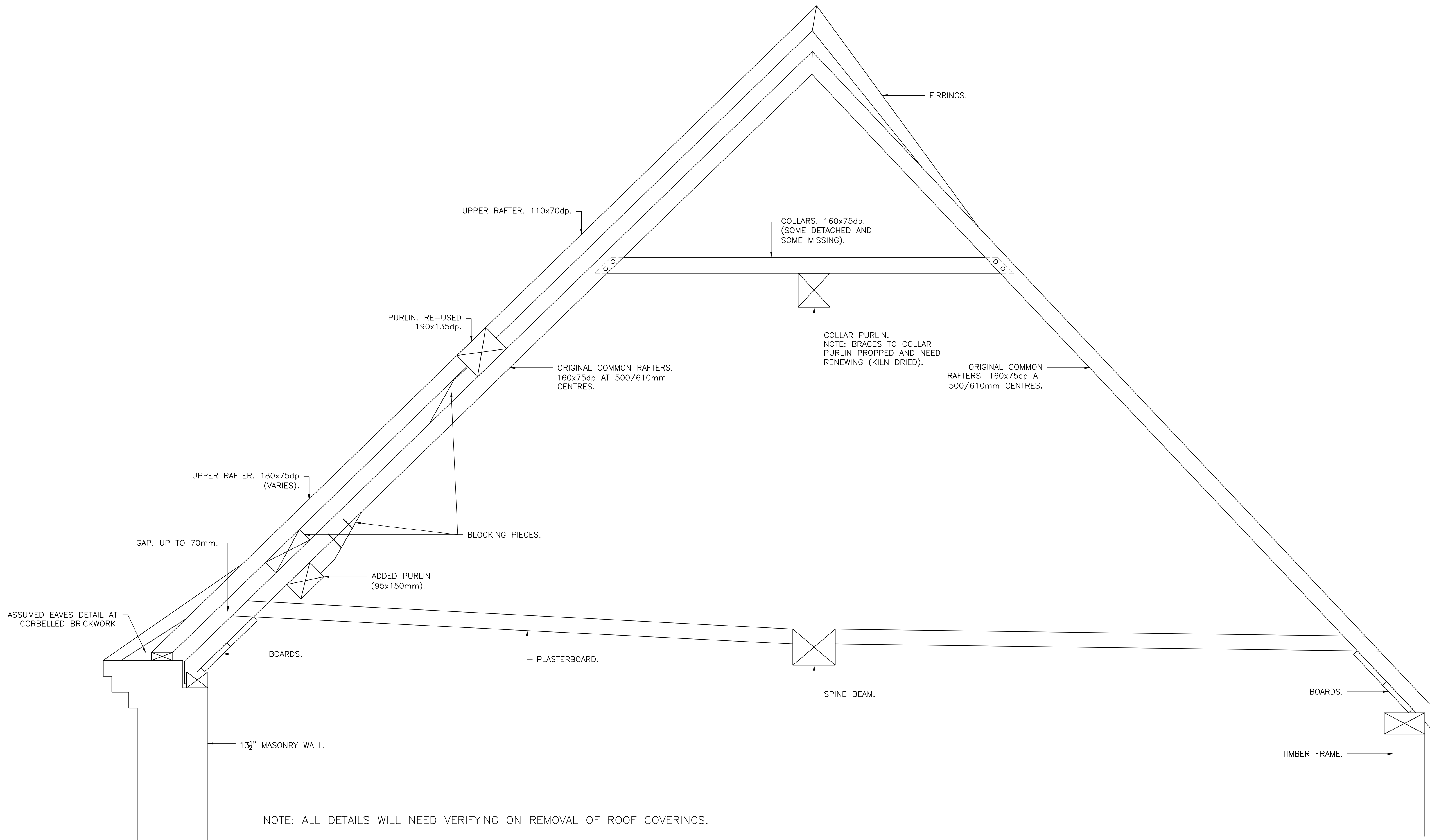
EXISTING SECTION (THROUGH NORTH BAY 5) SCALE 1:10
