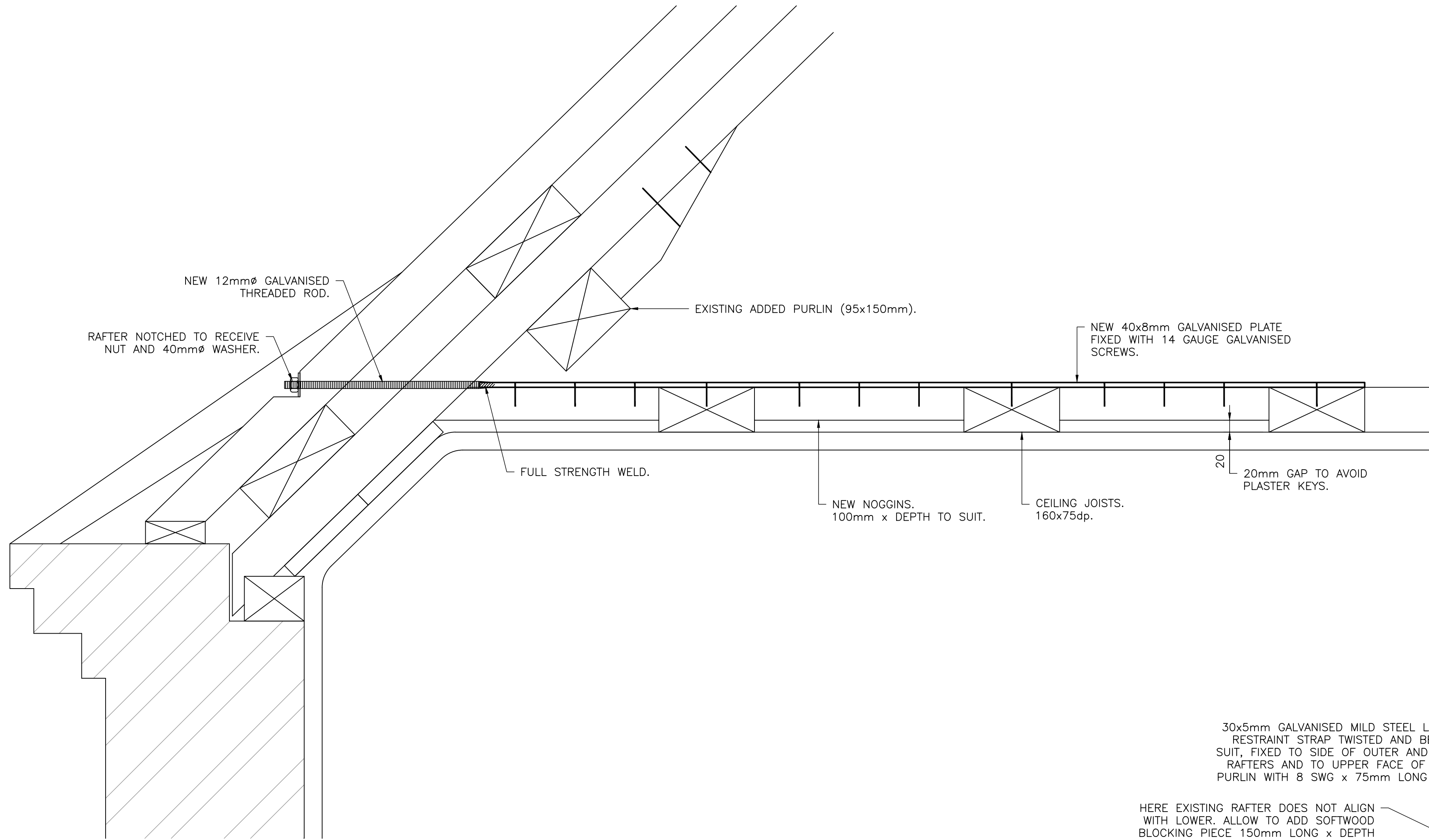
PROPOSED FRONT EAVES (BAY 4) SCALE 1:5
