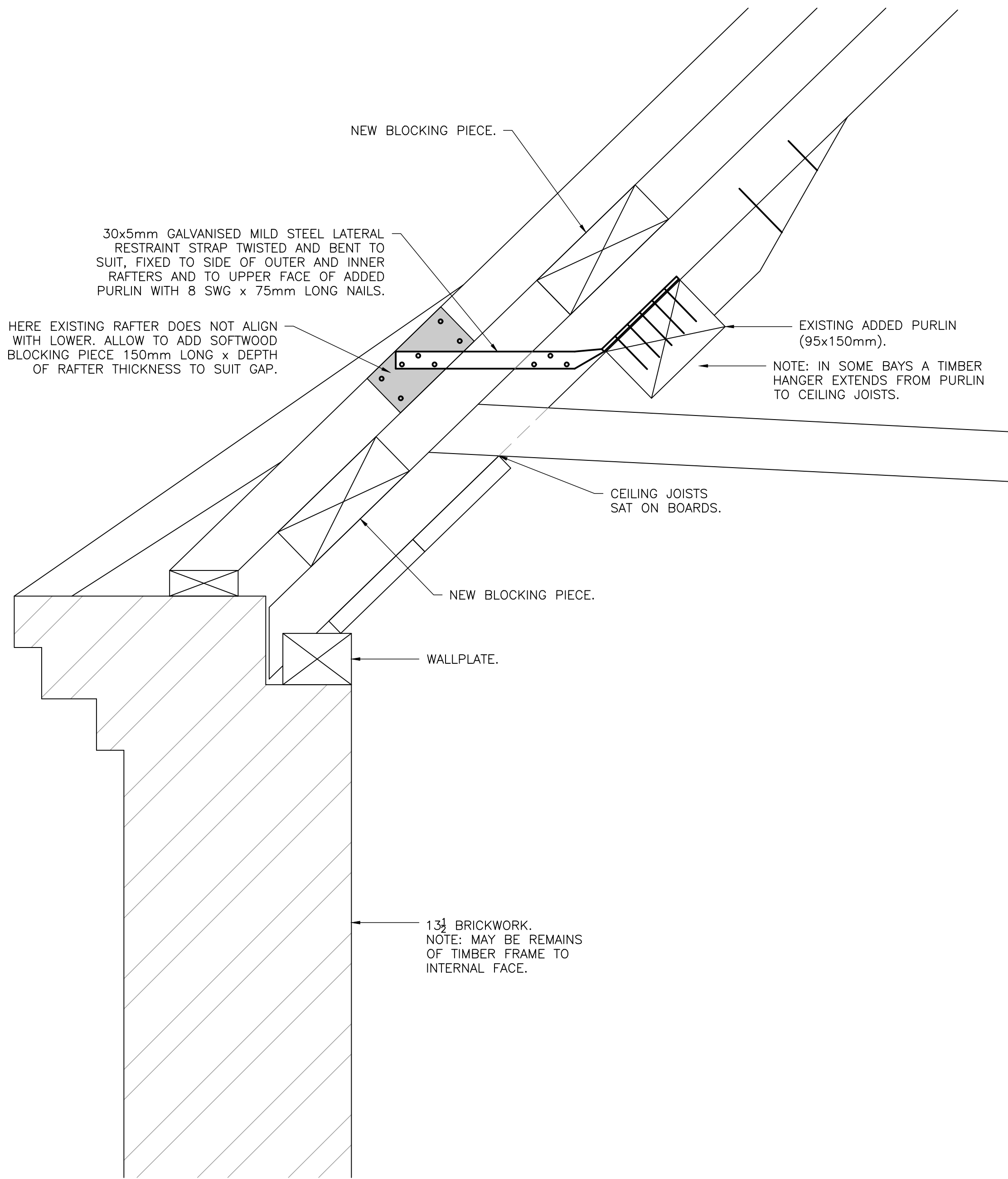
PROPOSED FRONT EAVES (BAYS 3 & 5) SCALE 1:5
