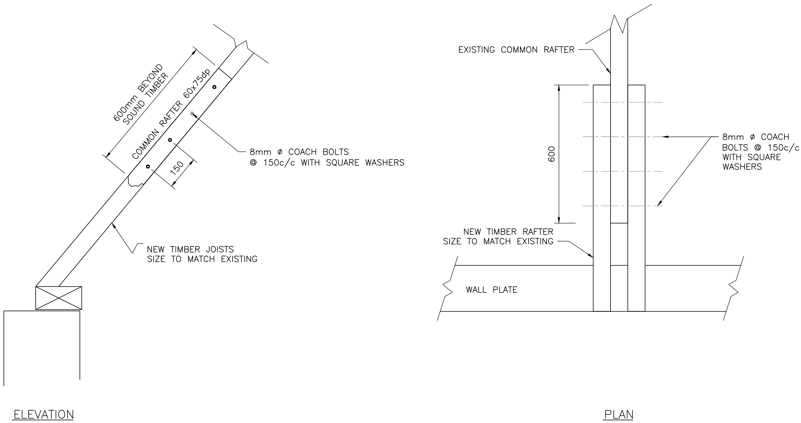
COMMON RAFTER SPLICE PARTNER DETAIL SCALE 1:10
