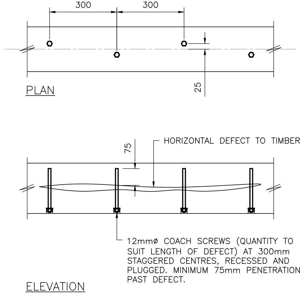
BOLT REPAIR TO HORIZONTAL DEFECT SCALE 1:10
