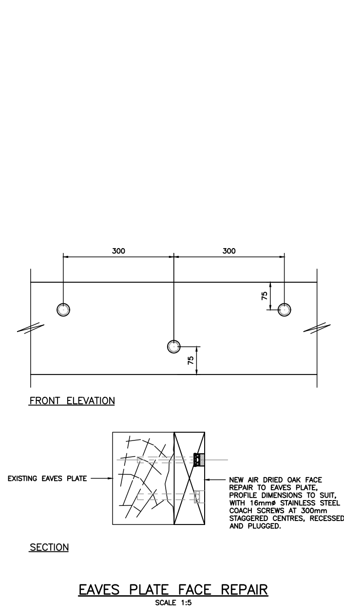
EAVES PLATE FACE REPAIR SCALE 1:5
