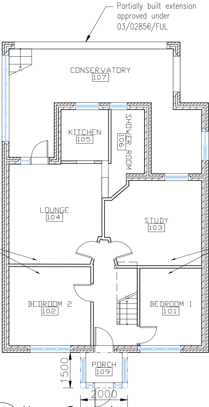
UG Upper Ground 1:100
