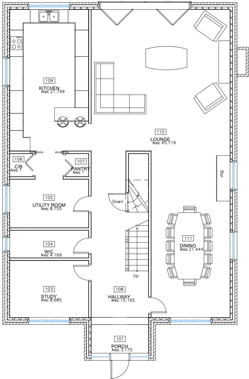
UG Proposed Upper Ground 1:100
