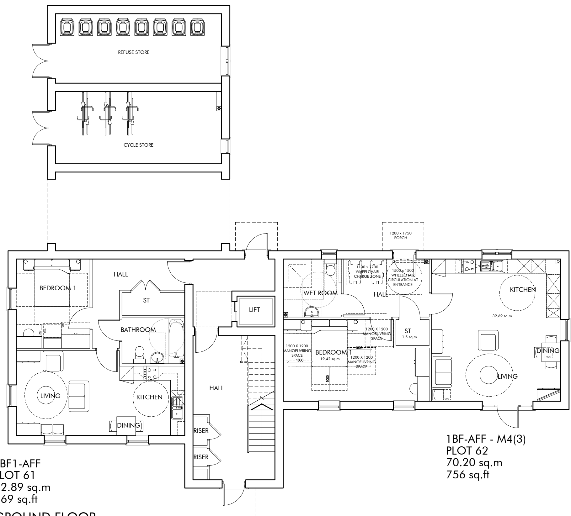
GROUND FLOOR
