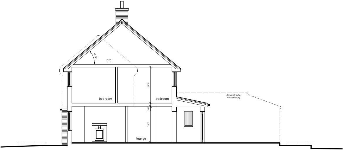
SECTION A
