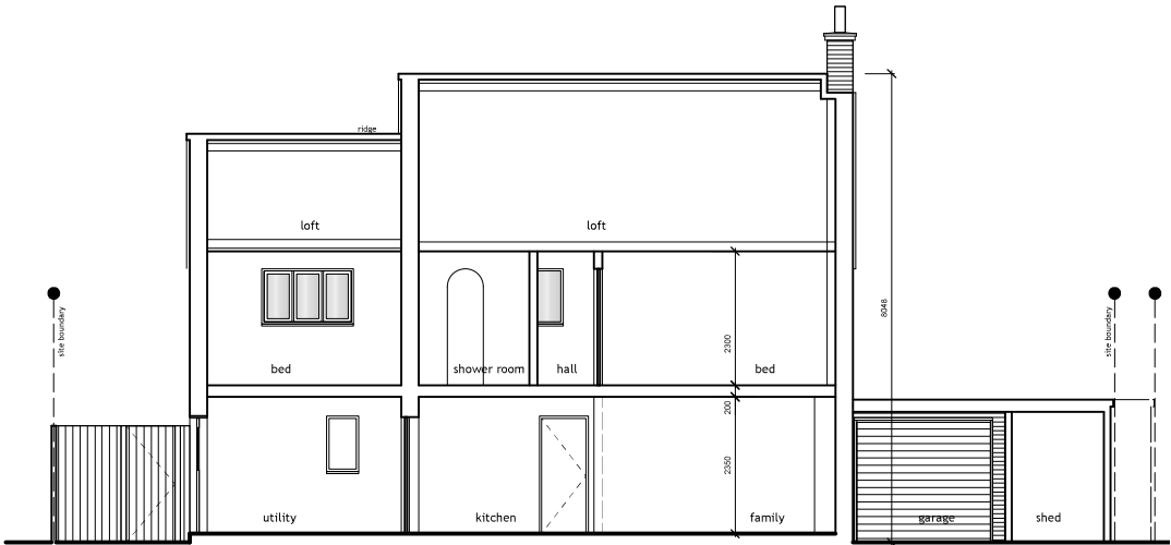
SECTION B
