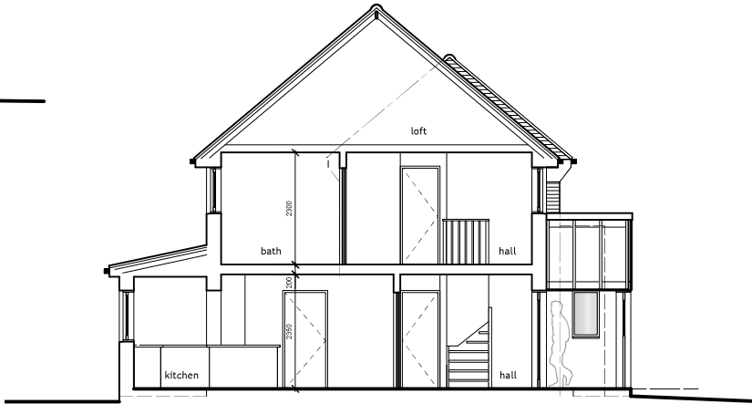
SECTION C
