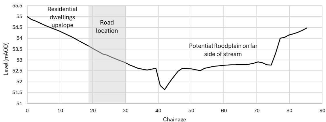
Figure 4-2 Typical cross-section through Site (near W2572)
