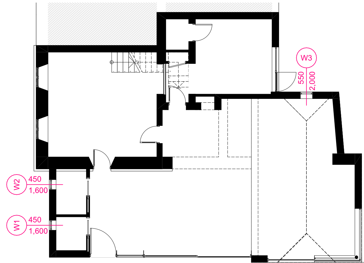
WINDOWS: GROUND FLOOR PLAN
