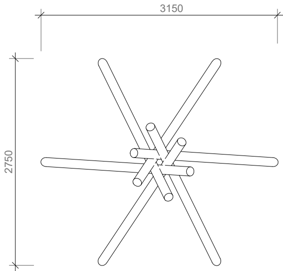
P-08 - Teepee Plan View
