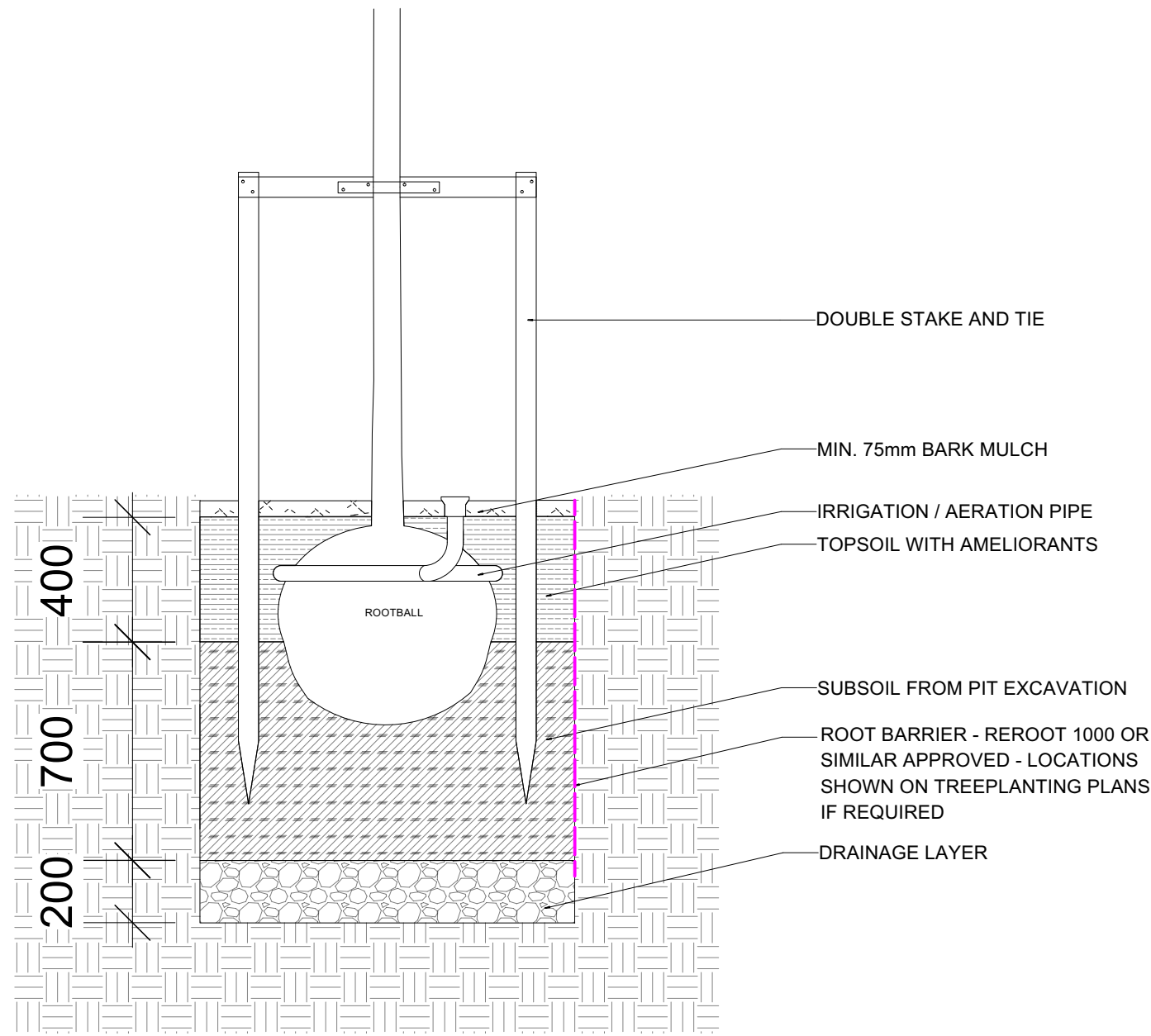
23-01 Tree pit type 1 - Section Scale: 1:20
