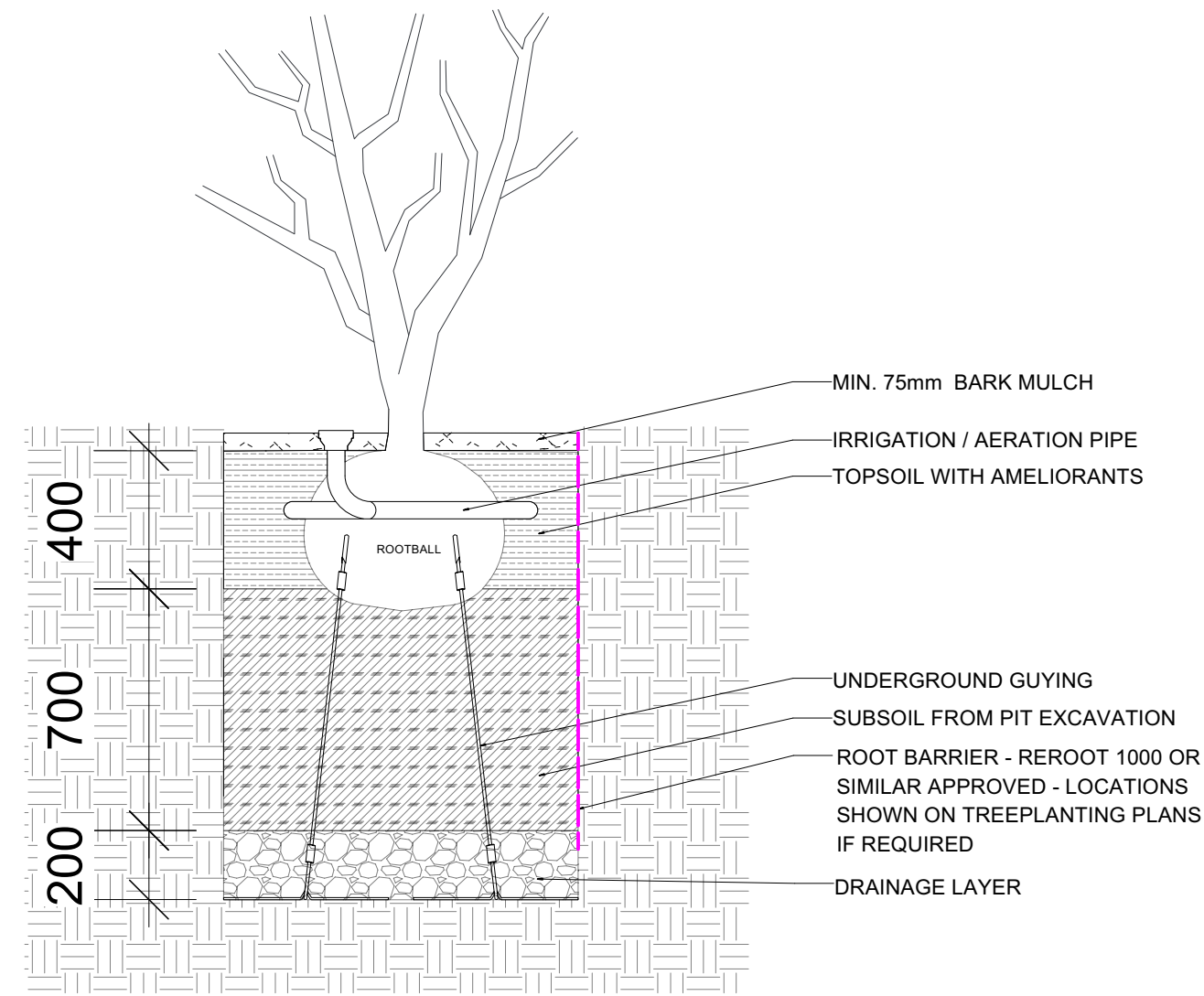
23-02 Tree pit type 2 - Section Scale: 1:20
