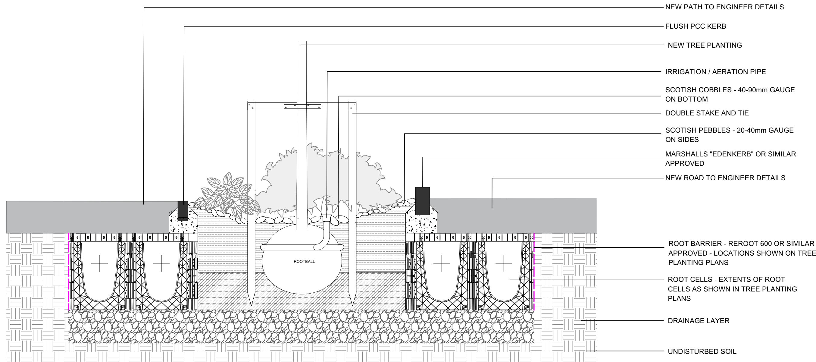
23-03 Tree pit type 3 - Section Scale: 1:20
