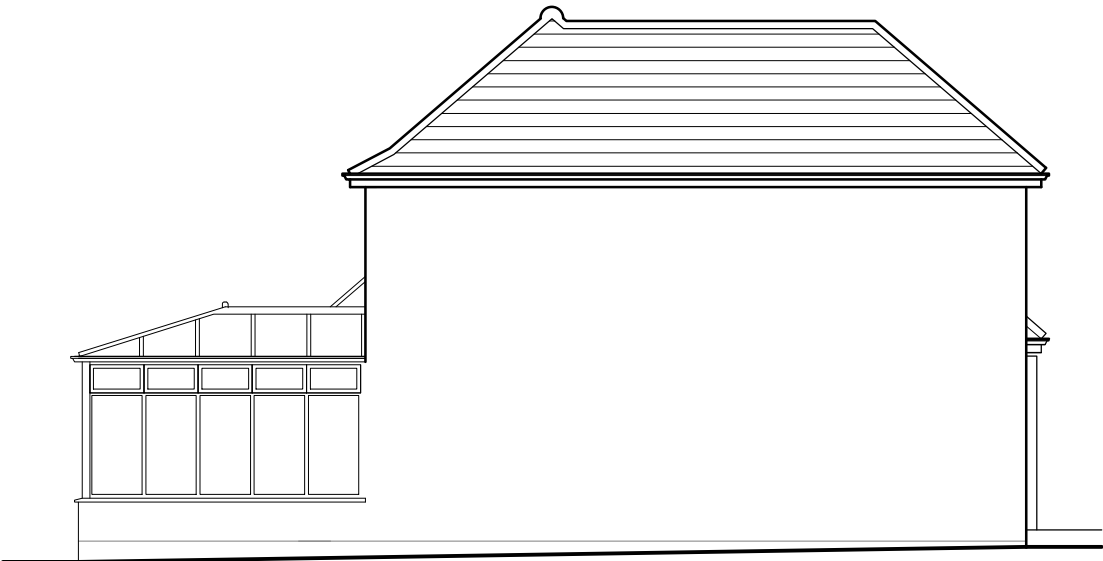
WEST ELEVATION AS EXISTING
