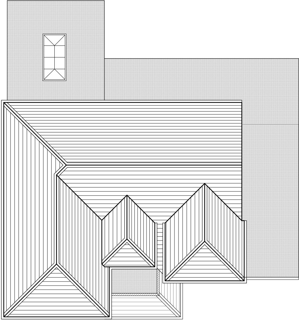
ROOF PLAN AS PROPOSED
