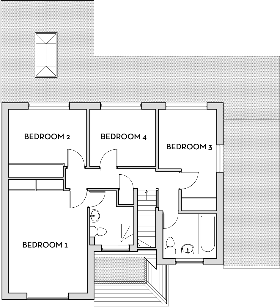
FIRST FLOOR PLAN AS PROPOSED
