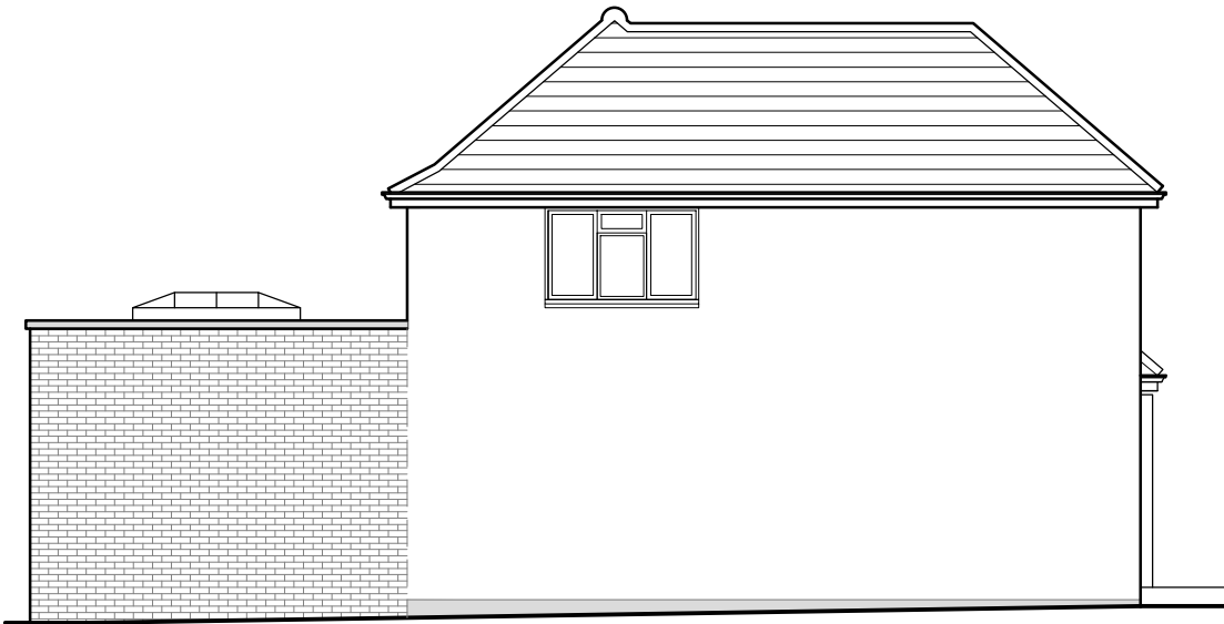
WEST ELEVATION AS PROPOSED
