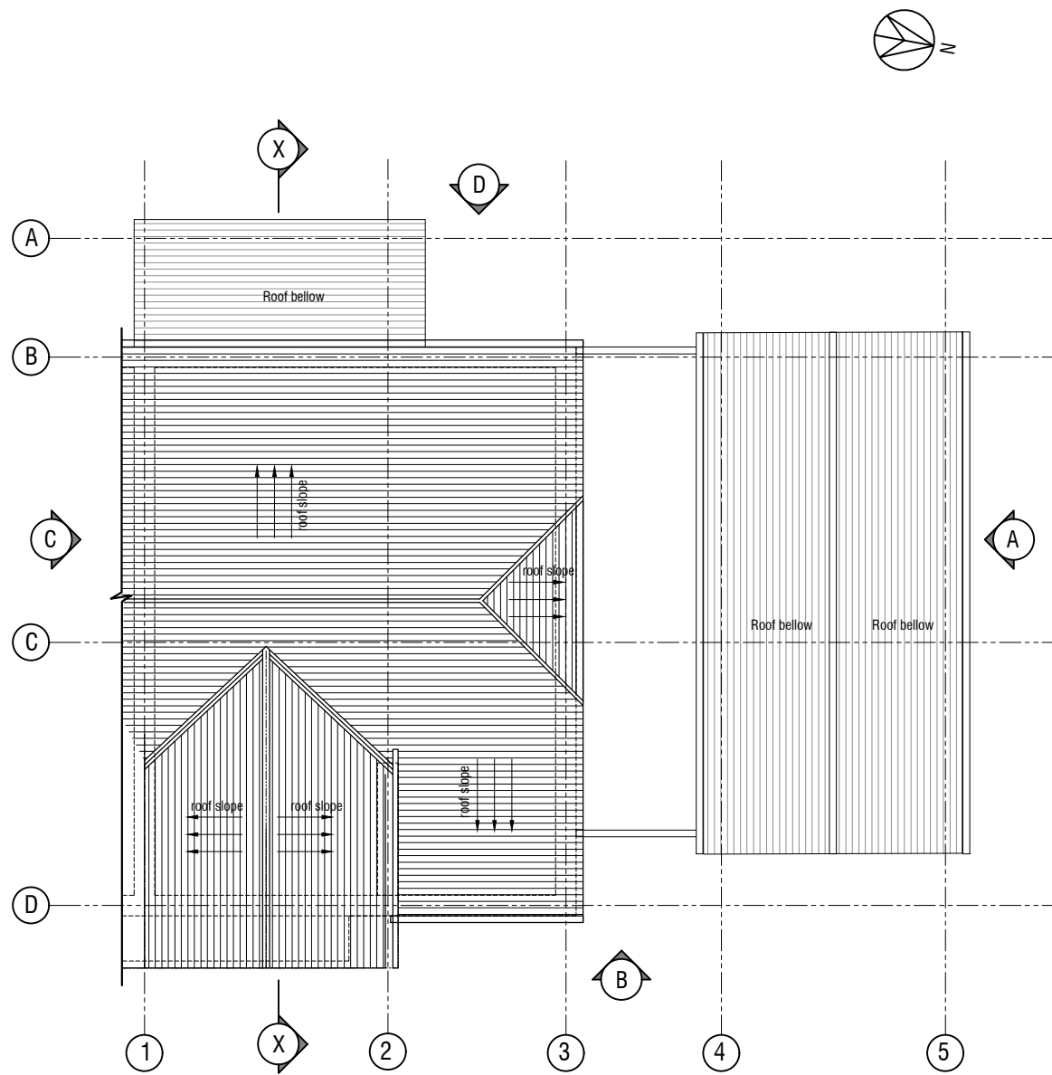
EXISTING ROOF PLAN Scale 1:100
