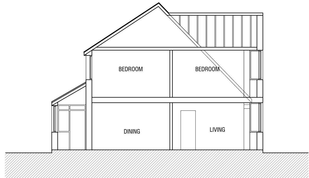
EXISTING SECTION XX Scale 1:100
