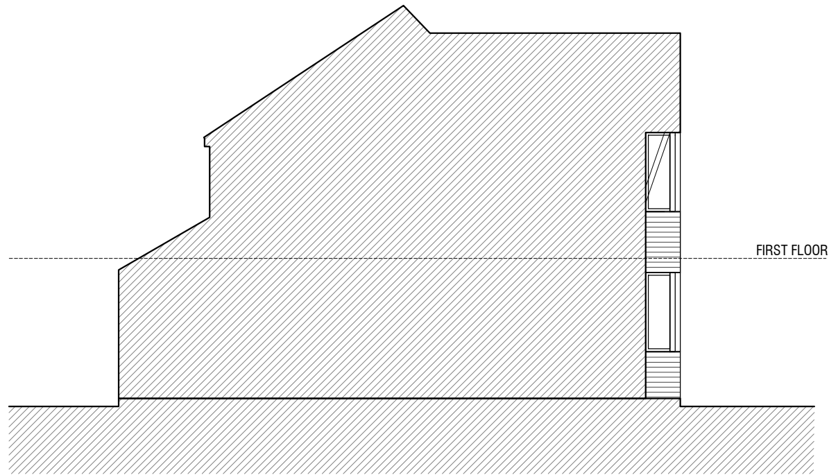
EXISTING SIDE ELEVATION C Scale 1:100
