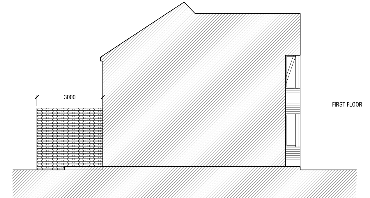
PROPOSED SIDE ELEVATION C Scale 1:100
