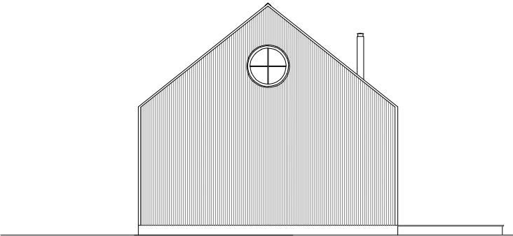
NORTH-WEST ELEVATION
