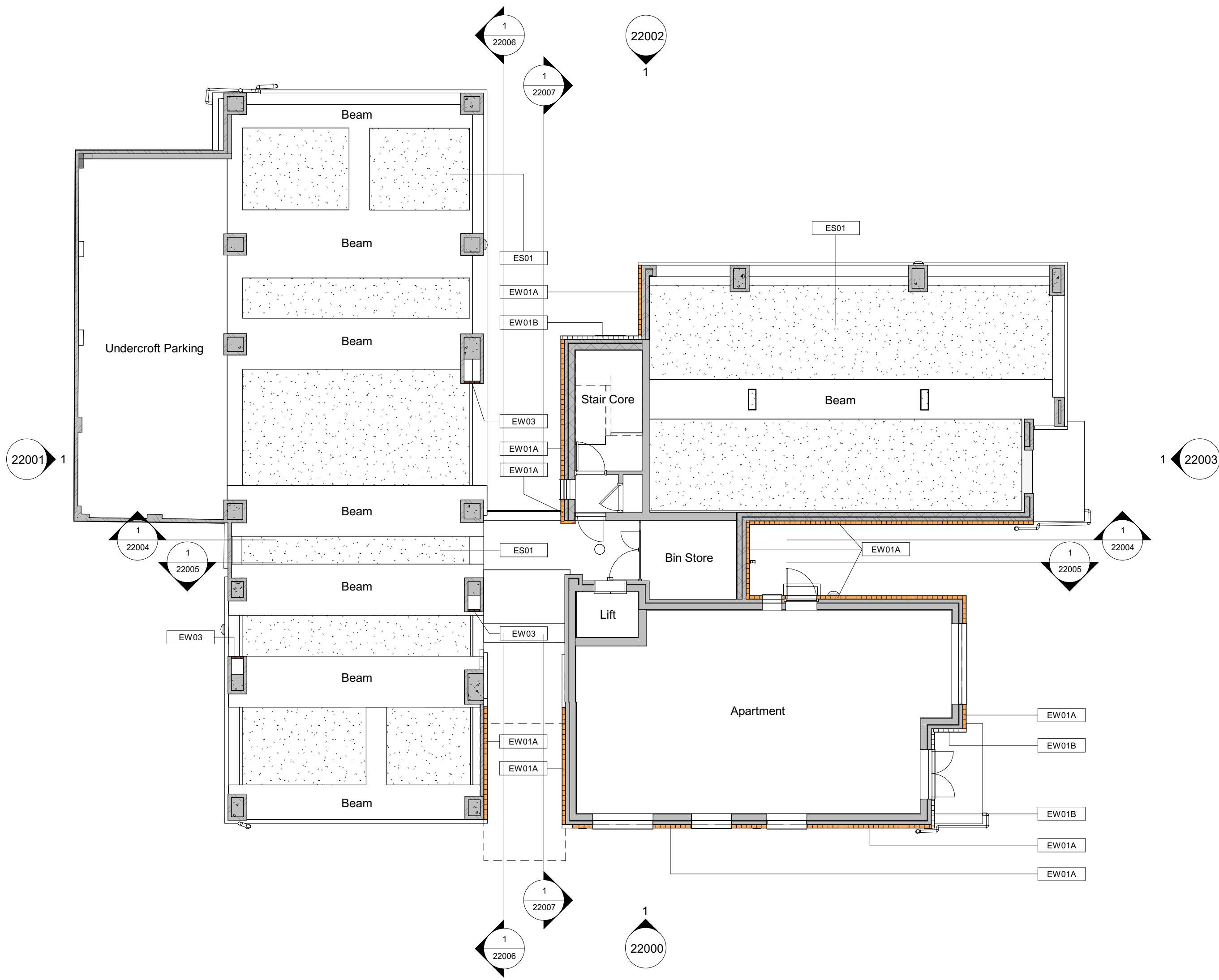
1 Planning - Existing Car Park Soffit 1 : 100
