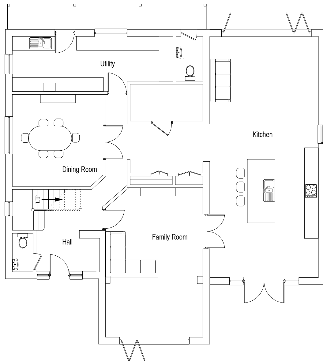
EXITING GROUND FLOOR PLAN
