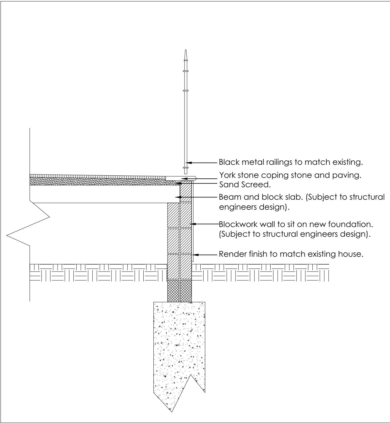
Section Detail As Proposed SCALE @ 1:20 ON AN A3 SHEET
