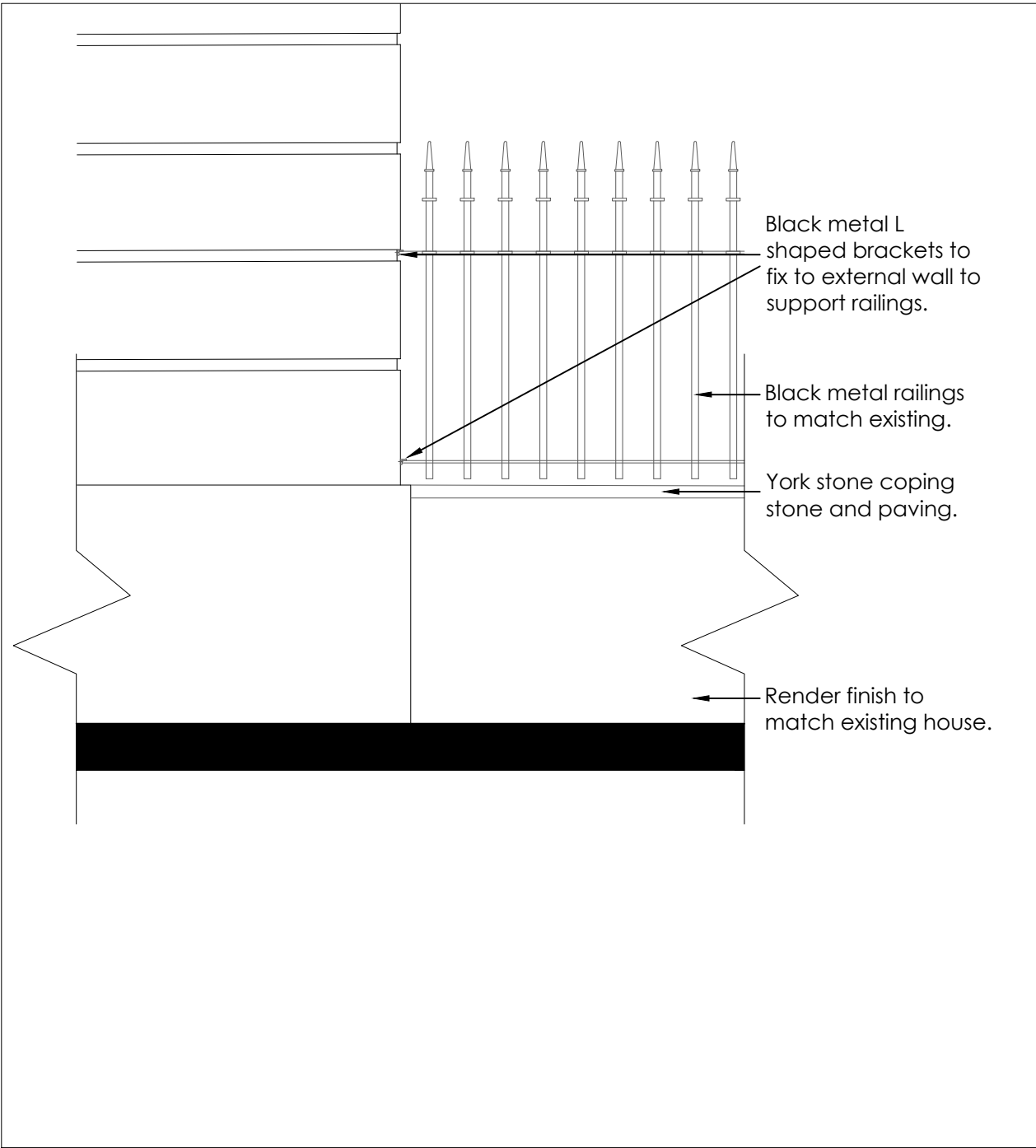
Elevation As Proposed SCALE @ 1:20 ON AN A3 SHEET
