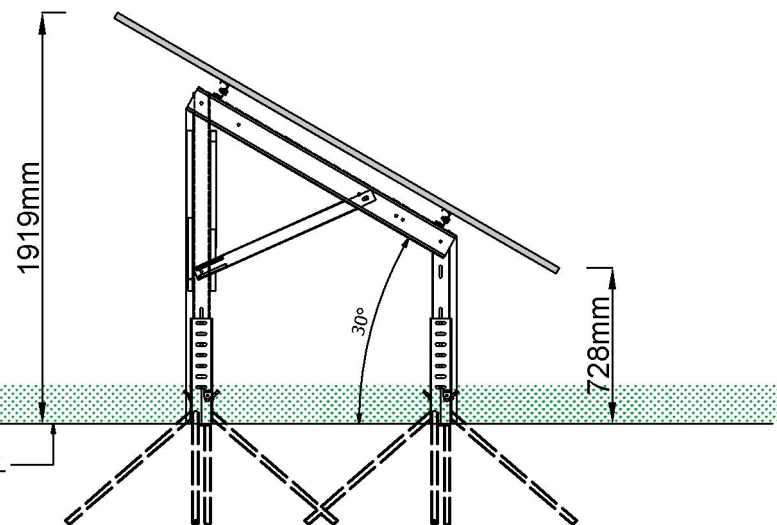
West Section
