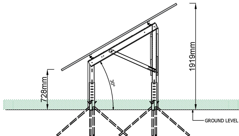
East Section
