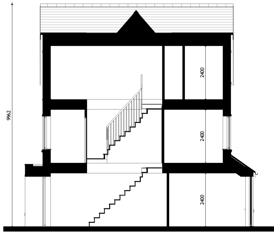
Building Section
