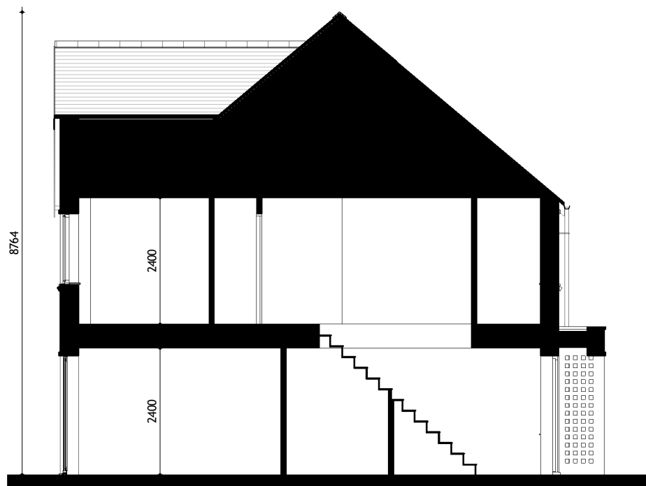
Building Section
