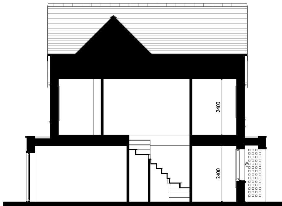
Building Section
