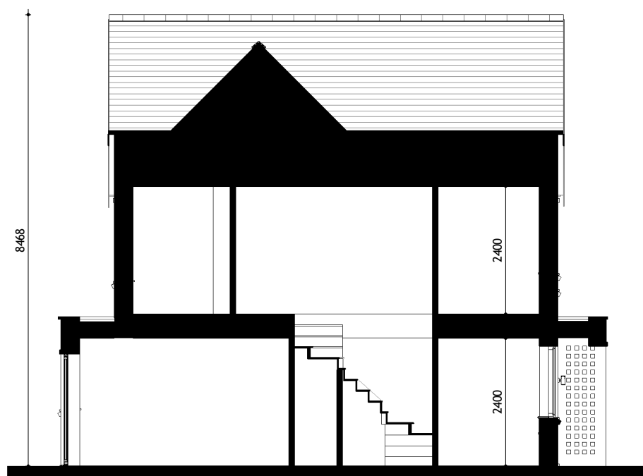
Building Section
