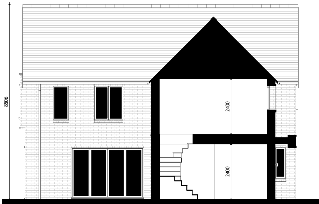
Building Section
