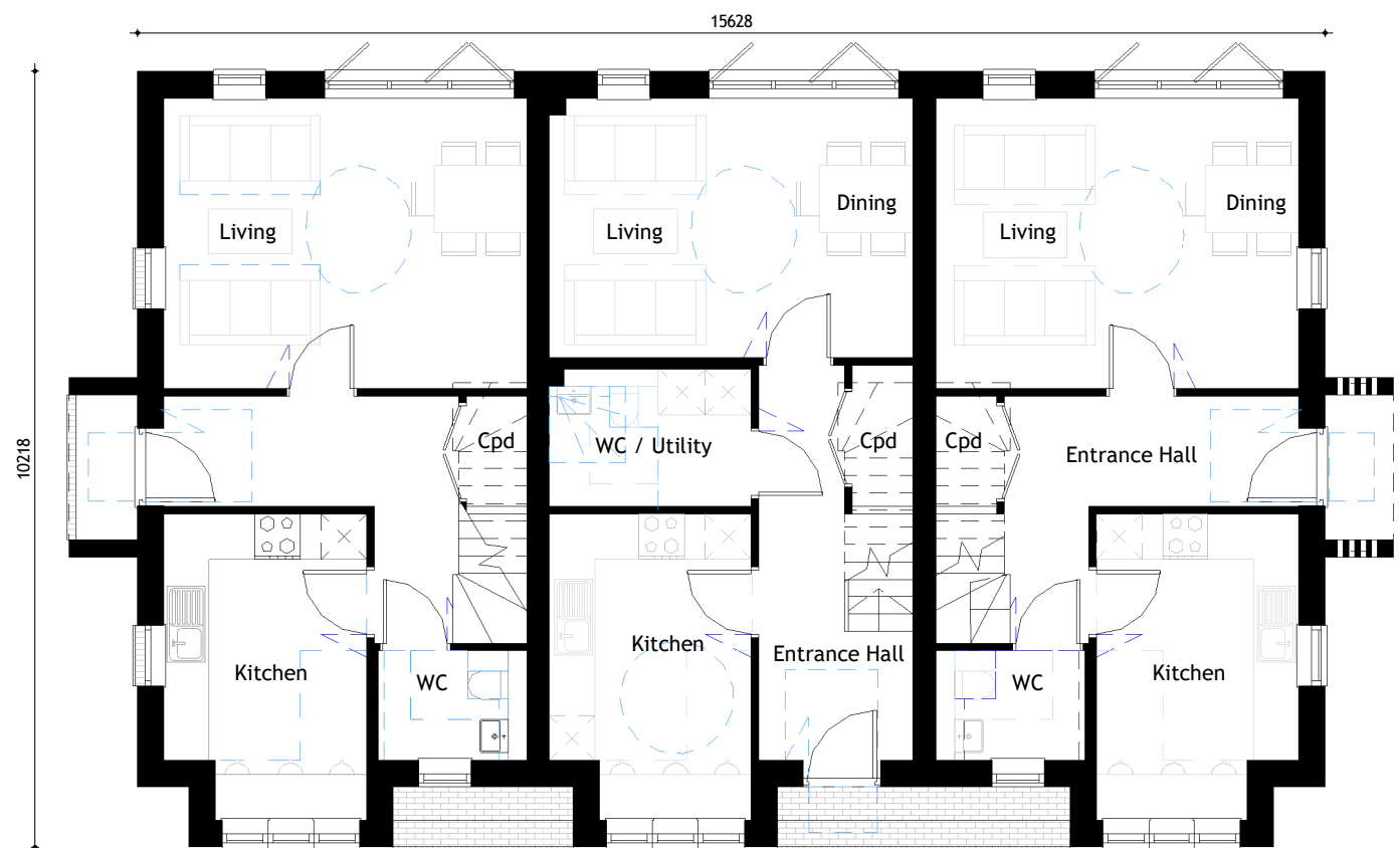
Ground Floor
