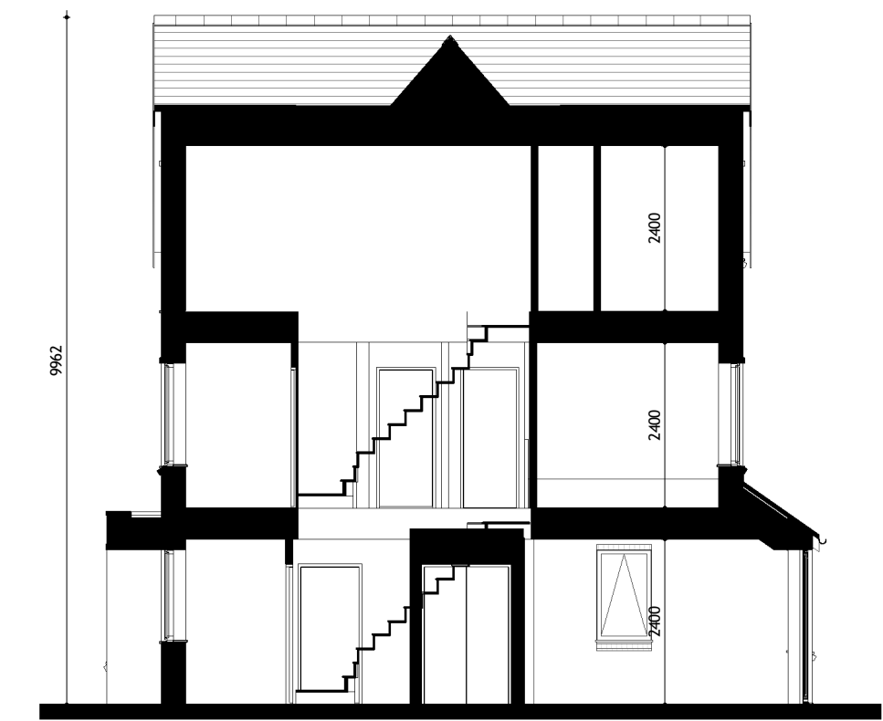
Building Section
