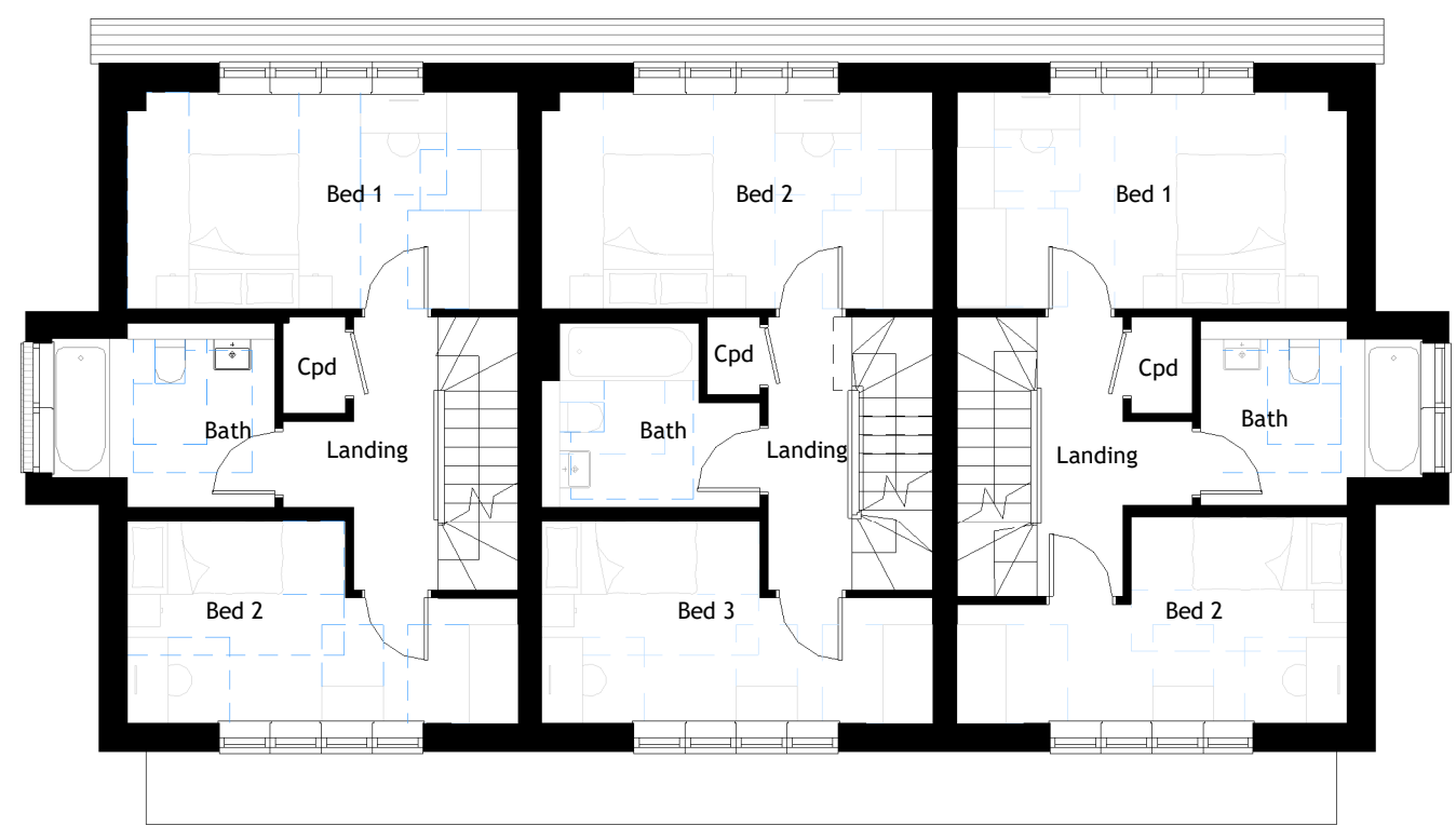
First Floor
