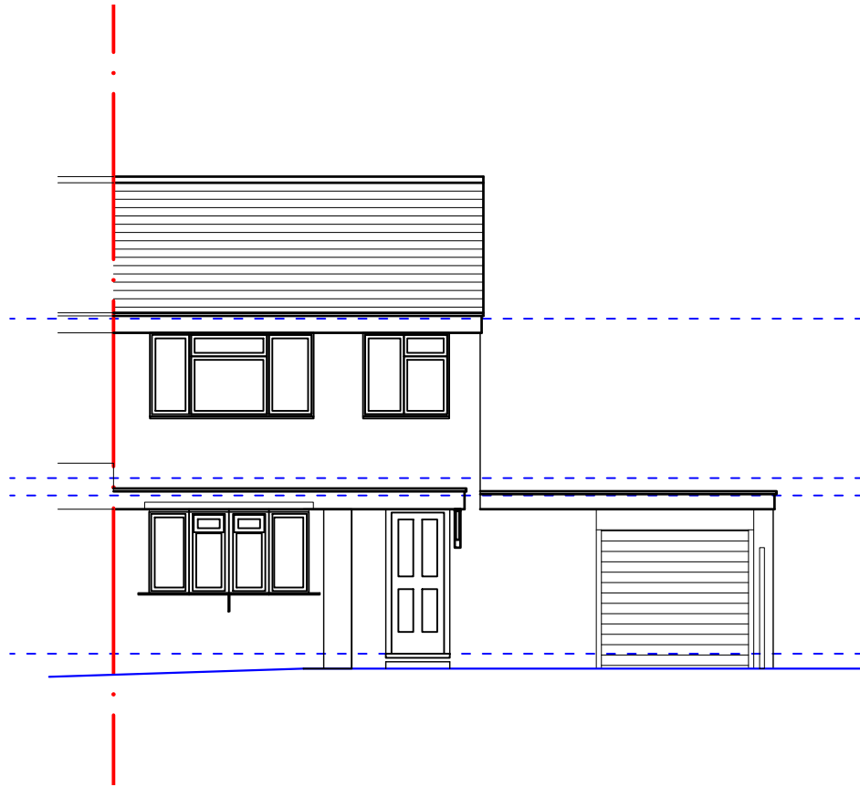
Existing Front (Northwest) Elevation 1:100@A3
