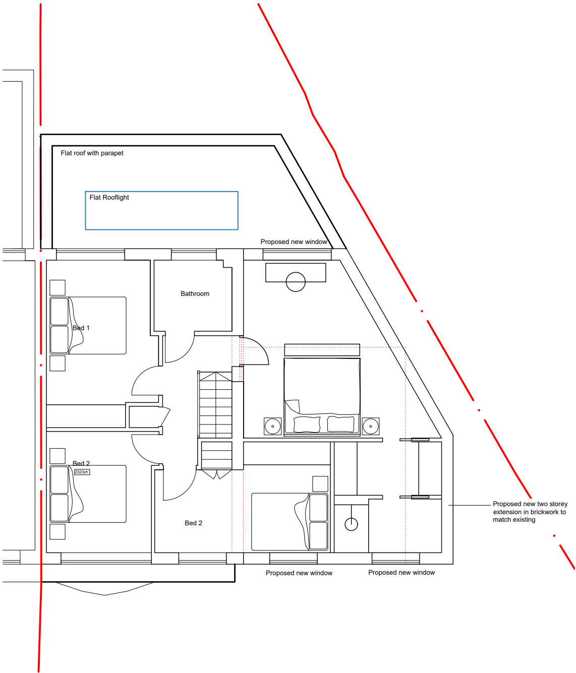
Proposed First Floor Plan 1:100@A3
