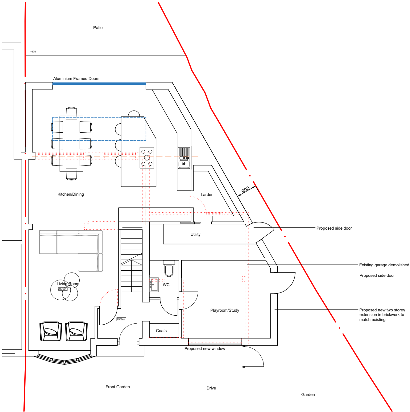
Proposed Ground Floor Plan 1:100@A3
