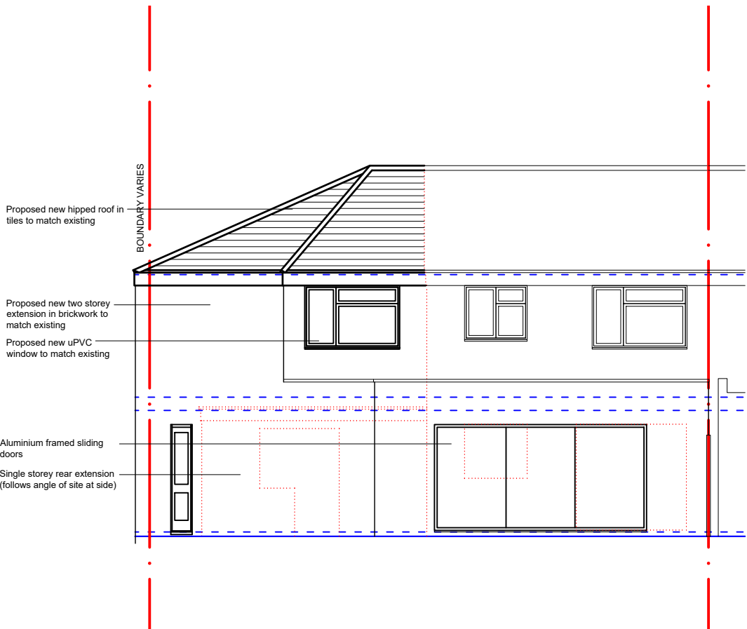
Proposed Rear (Southeast) Elevation 1:100@A3
