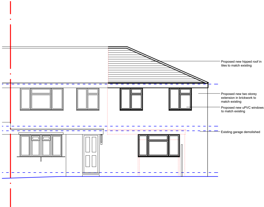
Proposed Front (Northwest) Elevation 1:100@A3
