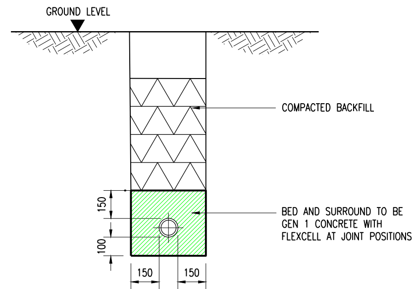
CLASS Z BEDDING: (WHERE COVER <600mm IN LANDSCAPED AREAS OR <900mm IN TRAFFICKED AREAS) (1:20)
