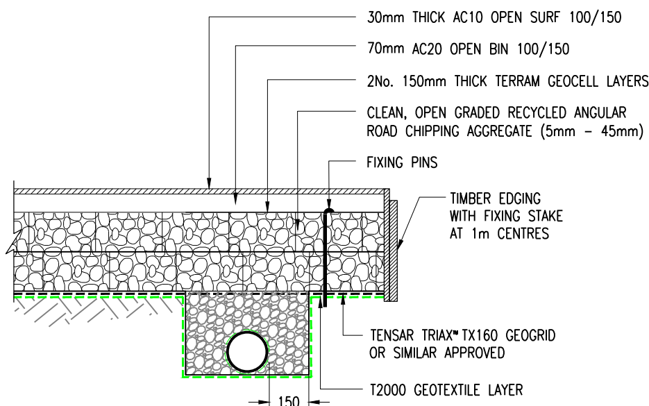
PERMEABLE SURFACE DETAIL (SHOWING PERFORATED PIPE) (1:20)
