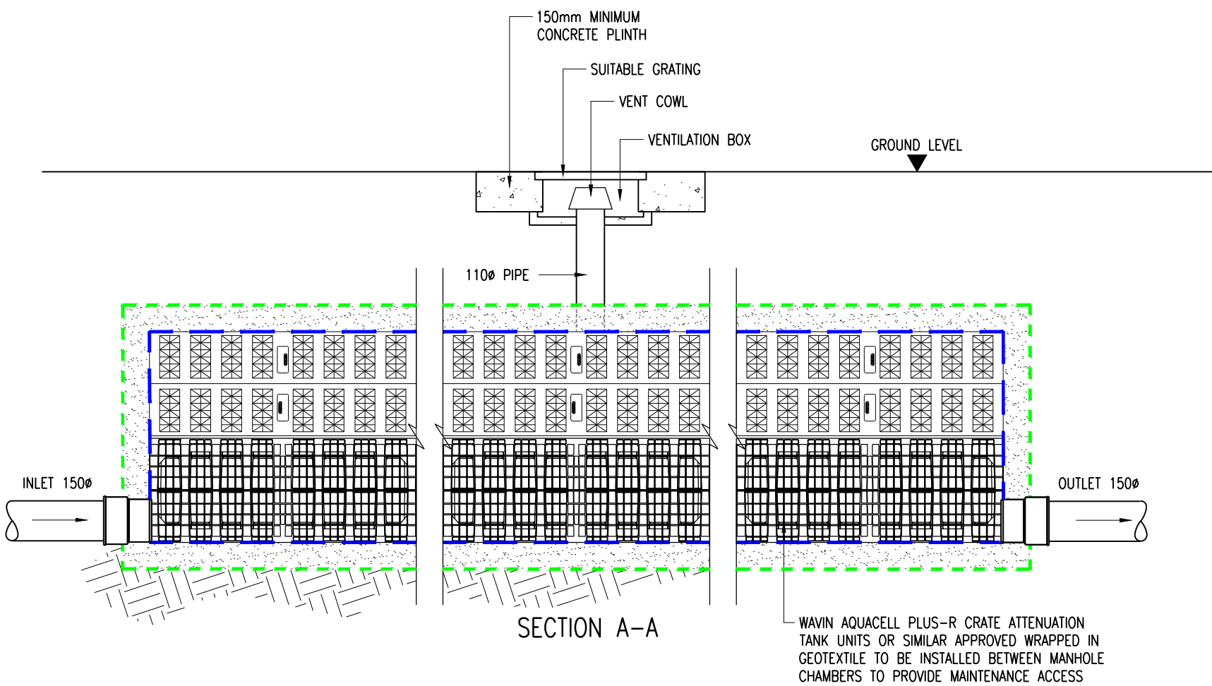
CRATE ATTENUATION TANK DETAIL (1:20)
