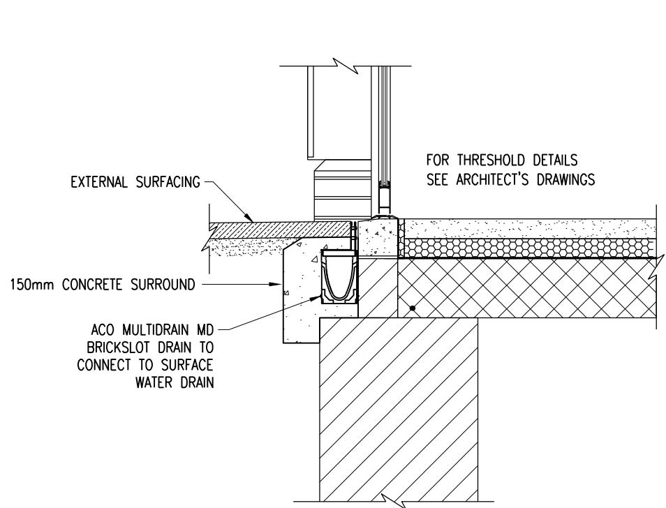
ACO BRICKSLOT DRAIN (AT THRESHOLD) (1:20)
