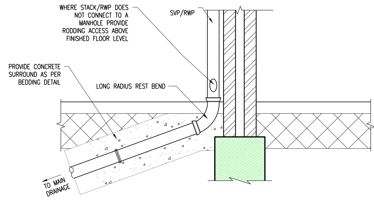
SVP/RWP CONNECTION (1:20)
