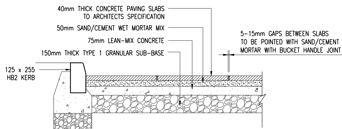
CONCRETE SLAB PAVING (TO PATIOS & PATHS) (1:20)
