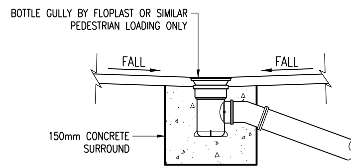
BOTTLE GULLY (1:20)
