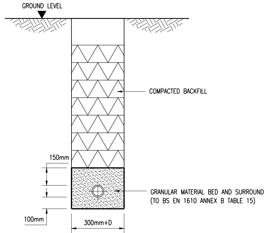
CLASS S BEDDING: (WHERE COVER >600mm IN LANDSCAPED AREAS OR >900mm IN TRAFFICKED AREAS) (1:20)
