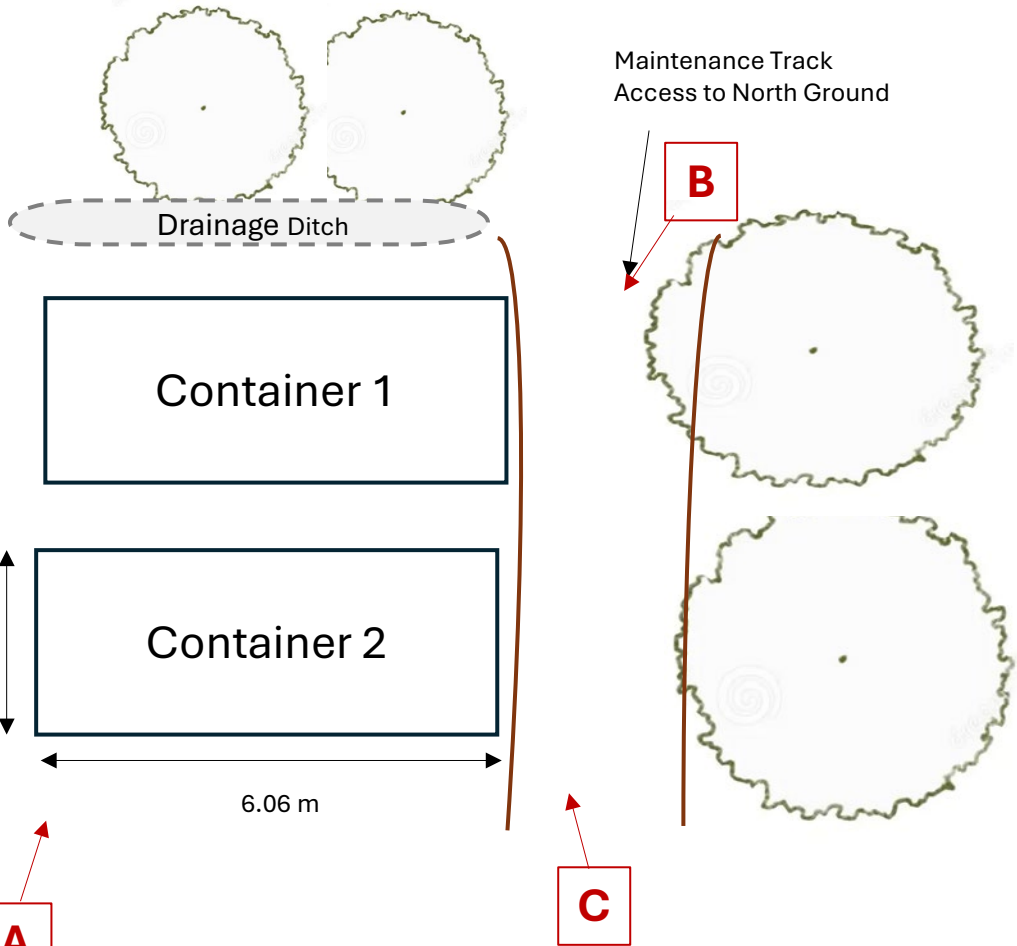
Plan Layout
