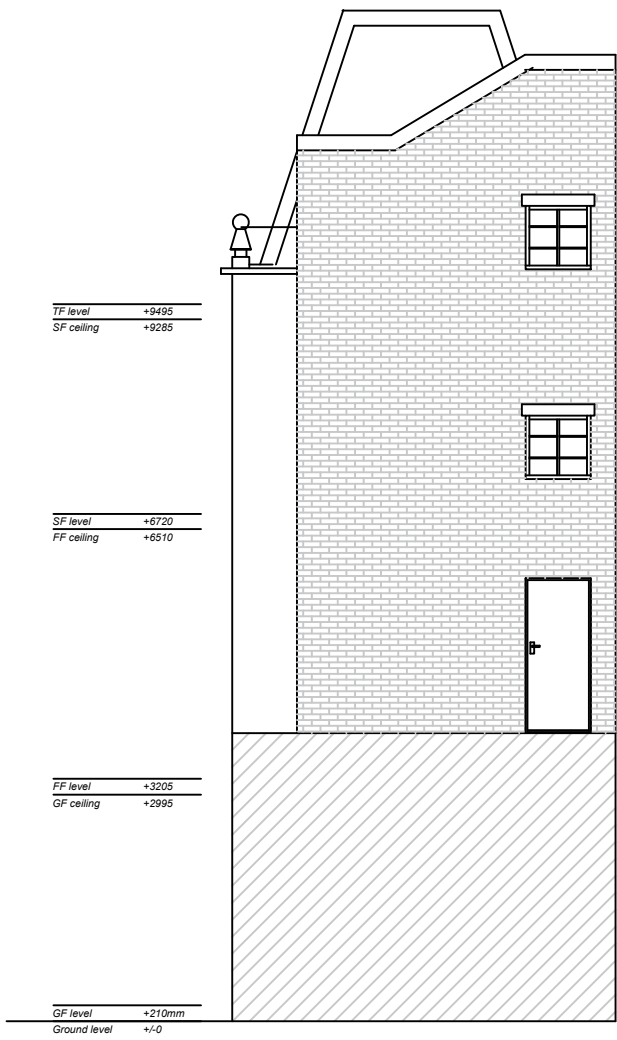
Rear Elevation
