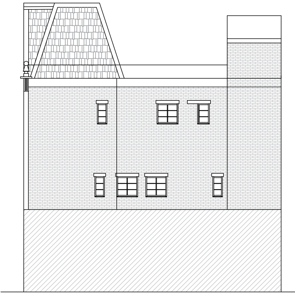
Side Elevation
