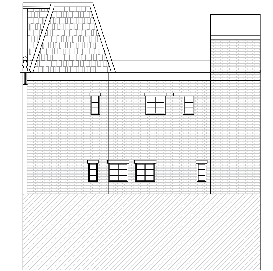
Side Elevation
