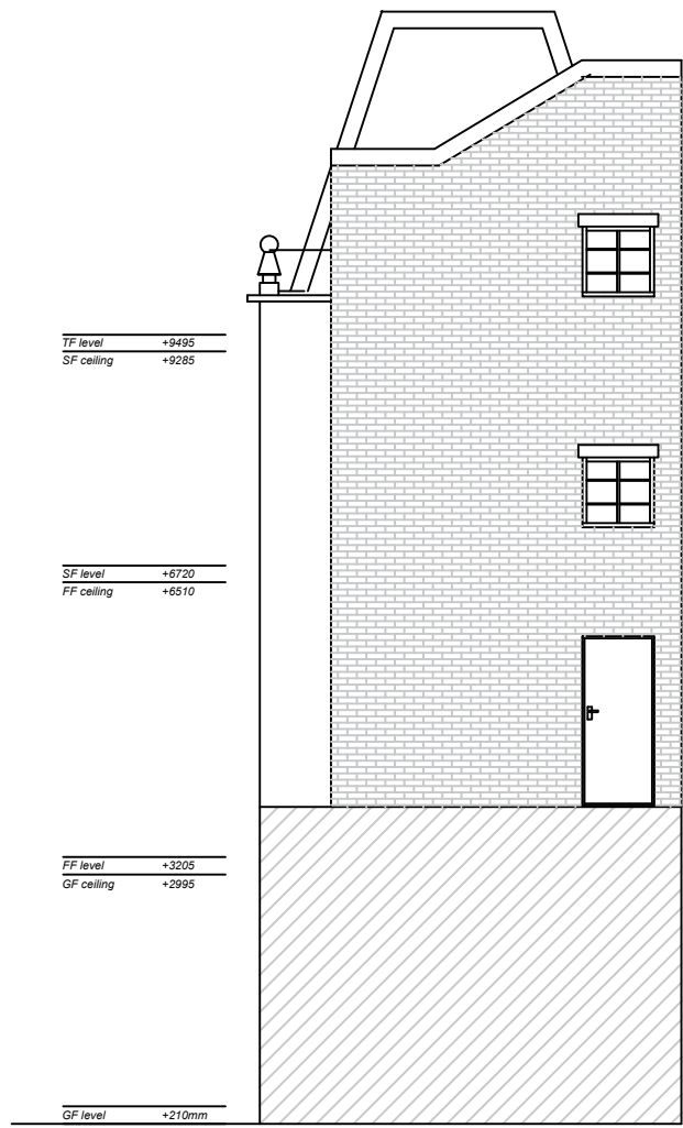
Rear Elevation
