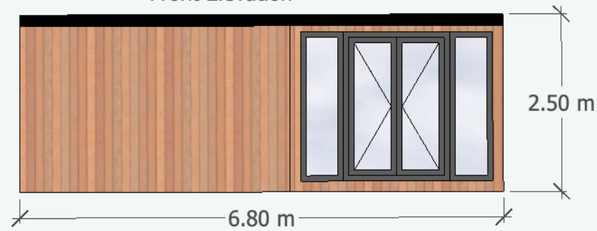
Front Elevation
