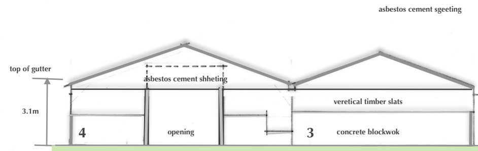
West Elevation
